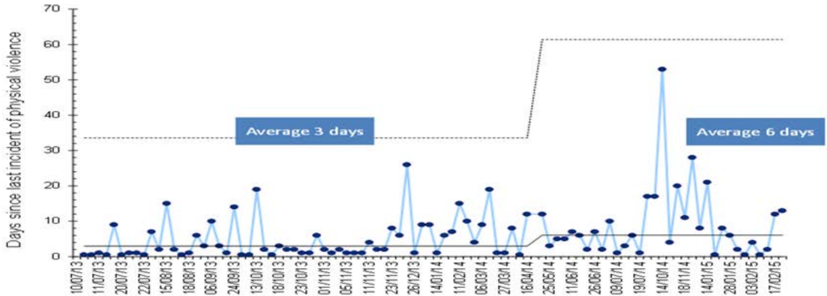
Days between staff injury due to physical violence (all three wards) - T Chart
