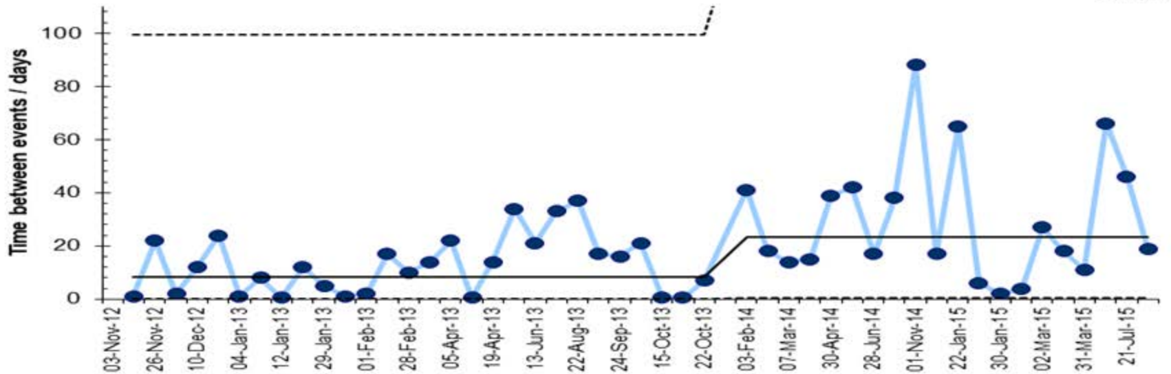
Days between staff injury due to physical violence (all three wards) - T Chart
